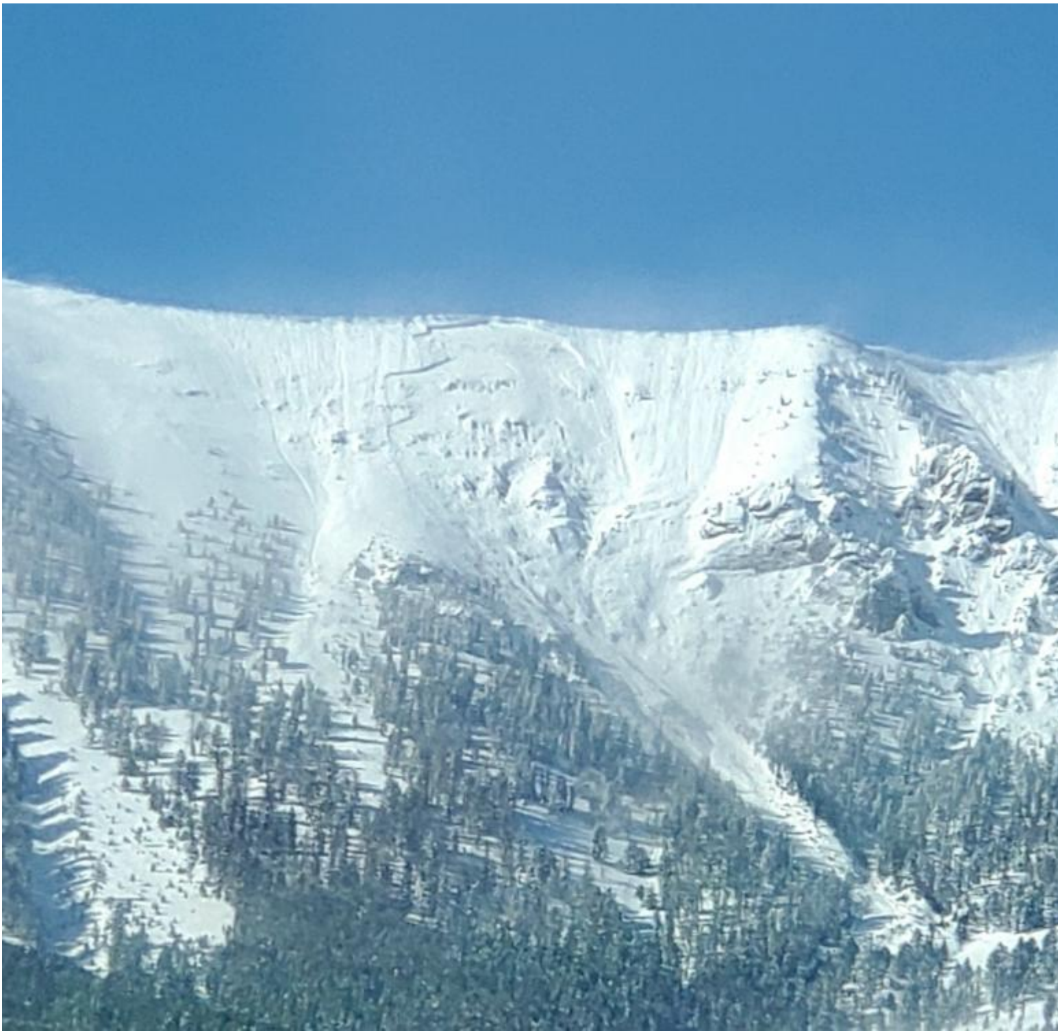
Natural avalanche south of Saddle Peak. 2/18/2021
